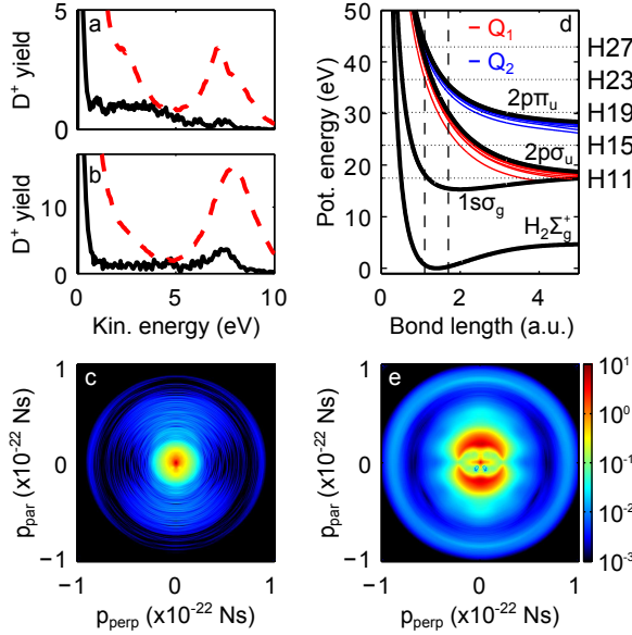
Figure 6.1: Fragment kinetic energy spectra from dissociative ionization of D_2 at 0^\circ (a) and at 90^\circ (b) \pm 20^\circ with respect to the laser polarization by the APT only (black solid lines) and by the APT+IR (cycle averaged) at temporal overlap (red dashed lines). Corresponding momentum maps for the APT (c) and the APT+IR (e). In (d) a potential energy diagram of D_2 is shown indicating the relevant neutral (red and blue) and ionic (black) states. The Franck-Condon region is indicated by vertical dashed lines and the position of a selection of harmonic orders present in the experiment are marked with horizontal dotted lines.
