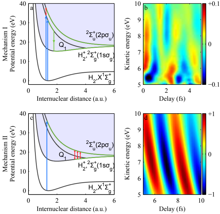
Figure 4.5: Asymmetry caused by the interference of a wave packet launched in the 2p\sigma_u state by direct XUV ionization or rapid ionization of the Q_1 \ ^1\Sigma_g^+ doubly-excited states by the infrared pulse and a wave packet in the 1s\sigma_g state resulting from autoionization of the Q_1 \ ^1\Sigma_g^+ states. Blue arrows indicate the effect of the XUV pulse and red arrows that of the infrared pulse; green lines and arrows signify dynamics that is intrinsic to the molecule. b, Close-coupling calculations in which direct photoexcitation to the 1s\sigma_g state has been excluded, supporting the notion that the Q_1 autoionizing states have an important role in the localization dynamics. c, Asymmetry caused by the interference of a wave packet that is launched in the 2p\sigma_u state by direct XUV ionization and a wave packet in the 1s\sigma_g state that results from stimulated emission during the dissociation process. d, Time-dependent asymmetry from a two-level calculation in which the wavefunction of the dissociating molecule is considered to be a coherent superposition of the 1s\sigma_g and 2p\sigma_u states.
