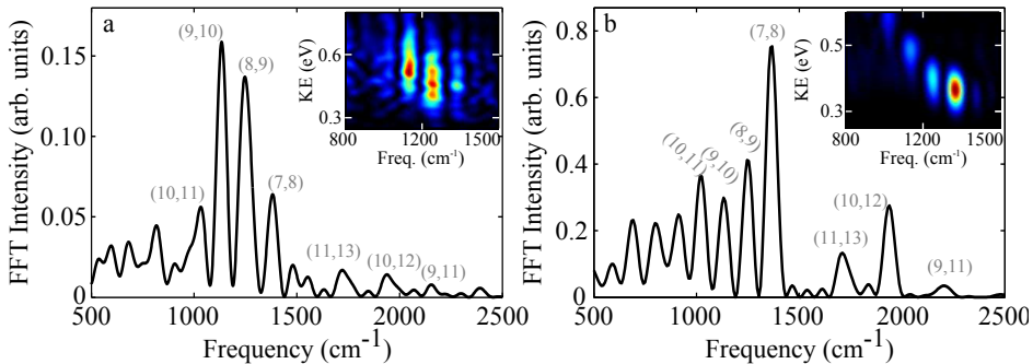
Figure 2.3: Fourier transform of the \text{H}^+ fragment yield integrated over the energy range between 0 and 1.2 eV for the experimental (a) and theoretical (b) results, in the case a 7 fs FWHM IR laser pulse. The spectra reveal the two-level beats [20] that are responsible for the observed time-dependence. The insets show an energy-resolved Fourier transformation and reveal a correlation between the fragment KE release and the vibrational level occupied prior to dissociation, observed both in the experiment and the simulations.
