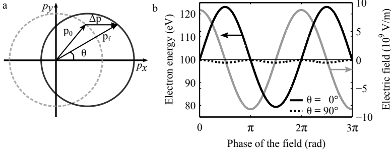
Figure 7.2: Principle of attosecond photoelectron streaking. (a) The dashed circle shows momentum distribution in the xy plane produced by the attosecond pulse which is shifted by \Delta \mathbf{p}(t_i) = -e\mathbf{A}(\mathbf{t}_i) through the interaction with the laser field. In (b) the resulting final energy W_f(t_i) for \theta = 0^\circ (solid black line) and for \theta = 90^\circ (dotted black line) is plotted as a function of the phase of the laser field together with the laser field with a wavelength of 800 nm and an intensity of 10^{13} \text{ W/cm}^2
