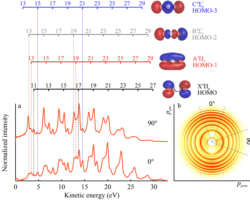
Figure 3.2: (a) Photoelectron spectra from randomly oriented CO 2 molecules for electrons emitted parallel ( \theta_e = 0^\circ ) and perpendicular ( \theta_e = 90^\circ ) to the polarization of the ionizing XUV pulse. (b) Photoelectron momentum distribution from which the spectra in (a) are obtained by integrating over a finite acceptance angle of \pm 20^\circ . The peaks in the spectra in (a) are the result of the presence of four ionization channels corresponding to the HOMO ( X^2\Pi_g , IP=13.8 eV), the HOMO-1 ( A^2\Pi_u , IP=17.6 eV), the HOMO-2 ( B^2\Sigma_u^+ , IP=18.1 eV) and the HOMO-3 ( C^2\Sigma_g^+ , IP=19.4 eV) orbitals of CO 2 . Each channel can be accessed by multiple harmonic orders in the XUV pulse as is indicated in the top part of the figure where the peak positions of the harmonic orders are given for the four ionization channels together with shape of the corresponding orbital.
