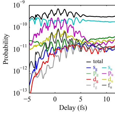
Figure 4.4: Angular momentum and electronic state-resolved delay dependence of H^+ ions with a fragment kinetic energy in the interval 7.5 \text{ eV} < E_k < 8.5 \text{ eV} . Angular momenta l_g and l_u respectively stand for l_g ; (1s\sigma_g\epsilon l)_g and l_u ; (2p\sigma_u\epsilon l)_u for l = 0 ( s_{g,u} wave), l = 2 ( d_{g,u} wave), ... (even l ) and l_g ; (2p\sigma_u\epsilon l)_g and l_u ; (1s\sigma_g\epsilon l)_u for l = 1 ( p_{g,u} wave), l = 3 ( f_{g,u} wave), ... odd l )
