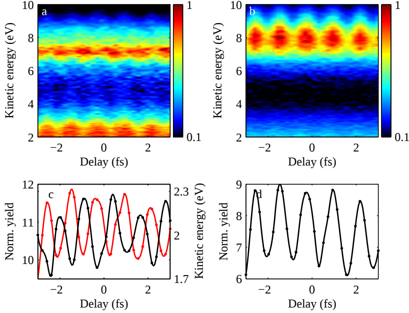
Figure 6.2: Time-dependent fragment kinetic energy spectrum as a function of delay \tau between the APT and the IR pulse for fragments ejected at 0° (a) and at 90° (b) \pm 20^\circ . In (c) and (d) ion yields as a function of delay are plotted for parallel and perpendicular fragments where the signal is normalized to the yield by the APT only of that particular channel. In (c) the black (red) curve is for fragments centered at 7 (3) eV and in (d) fragments around 8 eV are shown.
