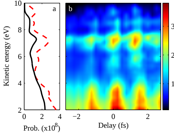
Figure 6.3: Results of the full calculations for dissociative ionization of D_2 by a 4-pulse APT and a 2.8 fs FWHM 780 nm field with a peak intensity of 3 \cdot 10^{12} \text{ W/cm}^2 . (a) Fragment kinetic energy spectra from the APT only (black solid line) and the APT+IR at \tau=0 (red dashed line) (b) Fragment kinetic energy spectrum as a function of delay between the two pulses.
