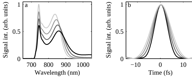
Figure 8.10: Spectrum (a) and fully compressed temporal profile (b) of the signal after amplification for different stretch factors of the signal input. The pump intensity is 9.8 GW/cm 2 with a pulse duration of 500 fs. The crystal length is 4 mm. The signal input is a 2 nJ pulse of 5 fs FWHM stretched to pulse durations of 50, 110, 180 and 280 fs with the darkest lines corresponding to the shortest input pulse. The plots show the trade-off between gain and bandwidth in the choice of the stretching factor, the larger the stretching factor the higher the gain but the smaller the bandwidth. The resulting pulse energies are 3.6 \mu J, 3.9 \mu J, 4.3 \mu J and 4.7 \mu J and the corresponding bandwidth limited pulse durations are 6.6 fs, 7.5 fs, 8.6 fs and 9.7 fs.
