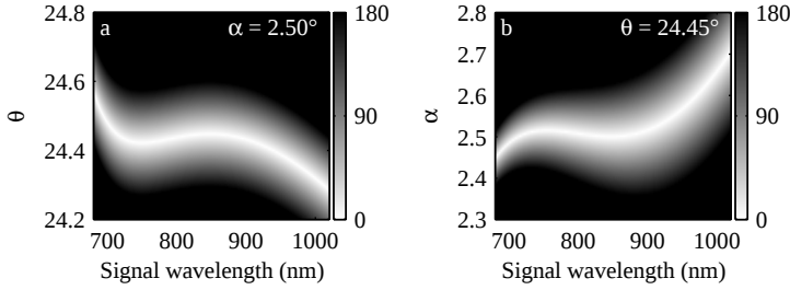
Figure 8.7: (a) Momentum mismatch \Delta k_{||} as a function of \theta and signal wavelength in type-I eoo phase matching with a non-collinear angle of \alpha = 2.5^\circ in units of degrees/mm crystal length. (b) Same plot as in (a) but now as a function of non-collinear angle \alpha for \theta = 24.45^\circ . Both plots show that phase matching over a large bandwidth (700-950 nm) can be achieved in a non-collinear geometry.
